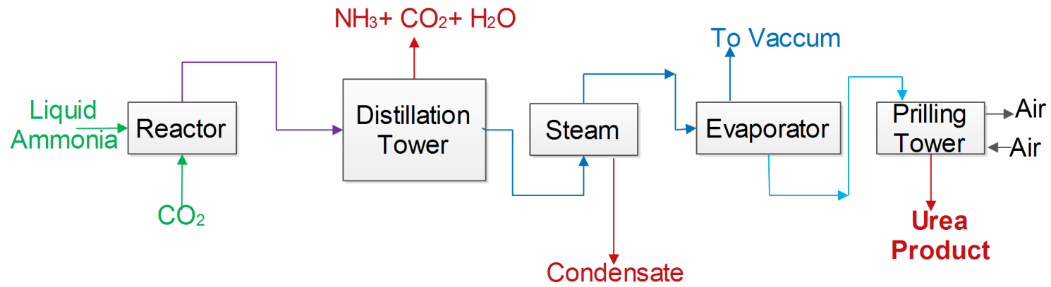
Figure: Manufacturing of Urea
